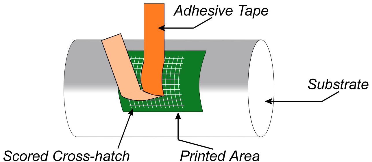
FIGURE 7. ADHESION TESTING
