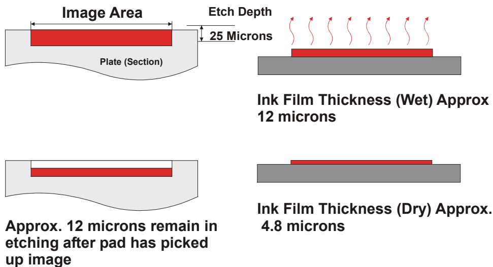
FIGURE 1. TYPICAL INK FILM THICKNESS
