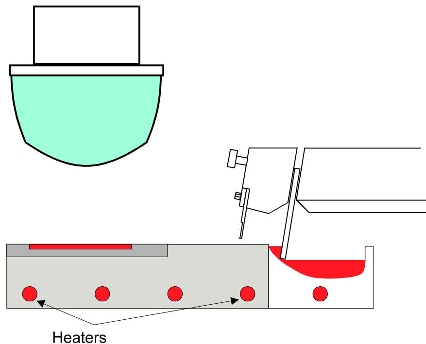
FIGURE 3. EXAMPLE OF INKING MECHANISM USED FOR PRINTING THERMOPLASTIC INKS
